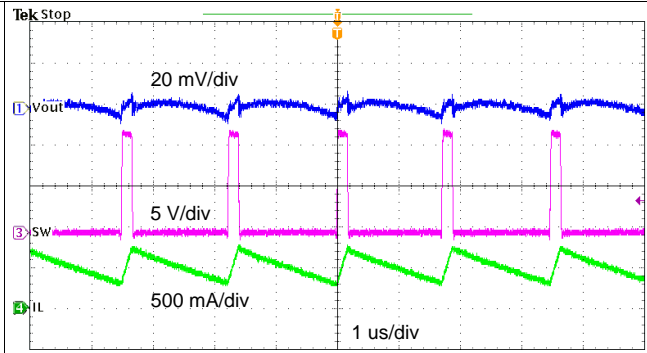
Figure 25. TPS561201 Output Voltage Ripple, I_{OUT} = 1 A
