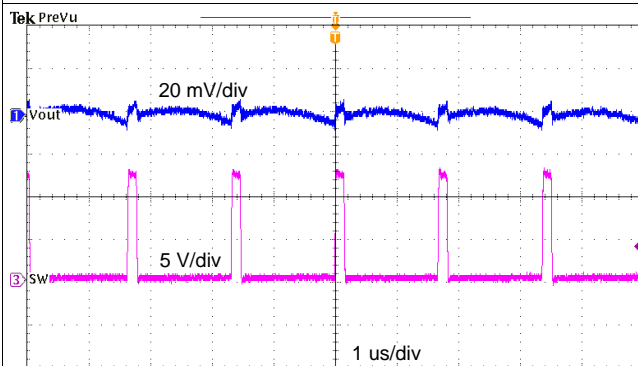
Figure 24. TPS561201 Output Voltage Ripple, I_{OUT} = 0.25 A
