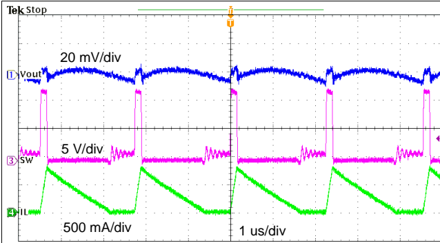
Figure 24. TPS561201 Output Voltage Ripple, I_{OUT} = 0.25 A
